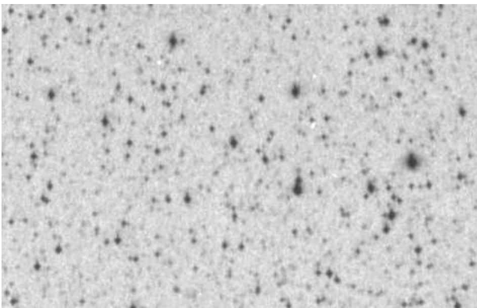
Platte 81 (300319) JD=2439531,31
